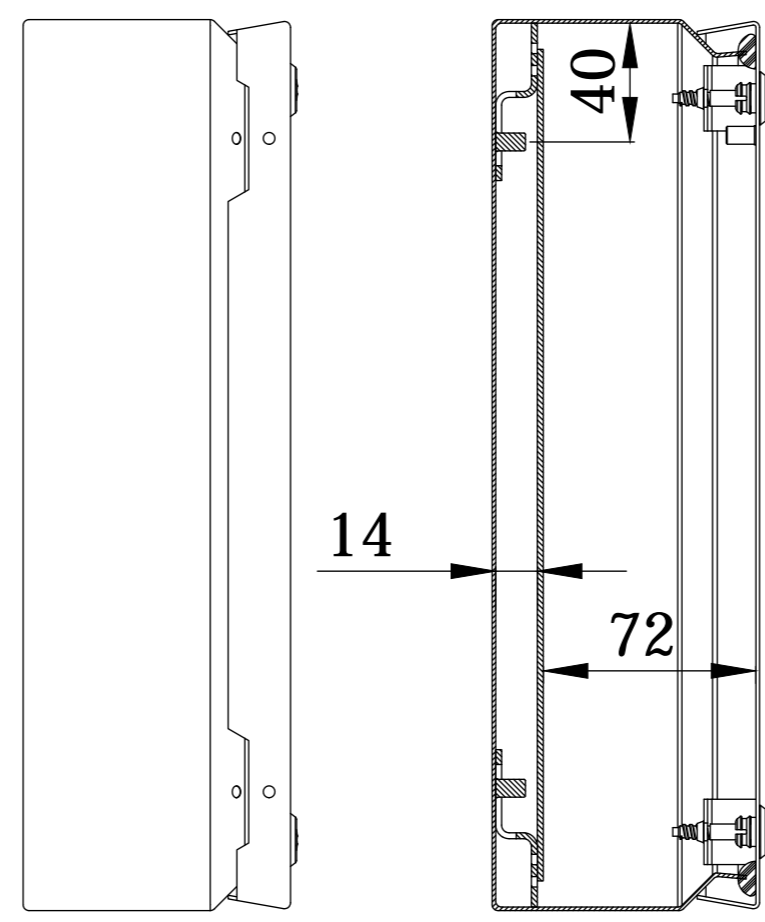
SEC.A-A'
