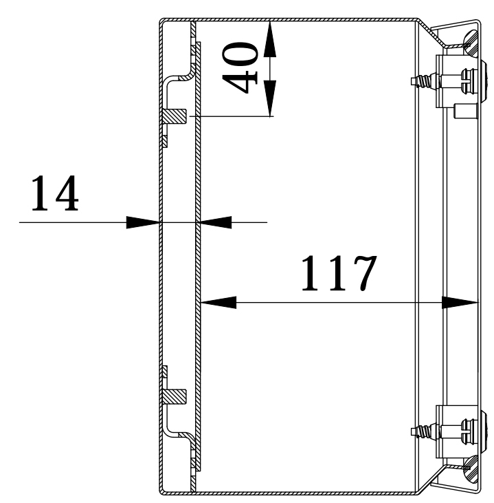
SEC.A-A'
