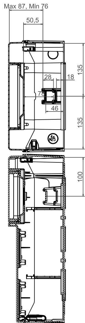
SEC AA
