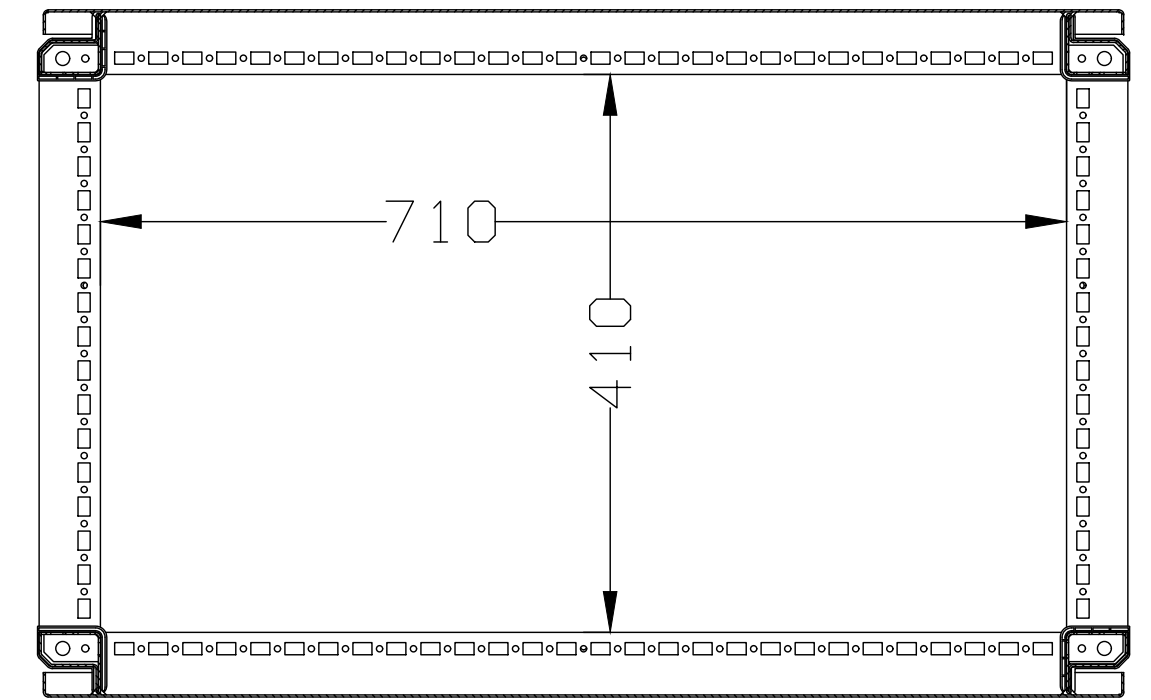
SEC. B-B
