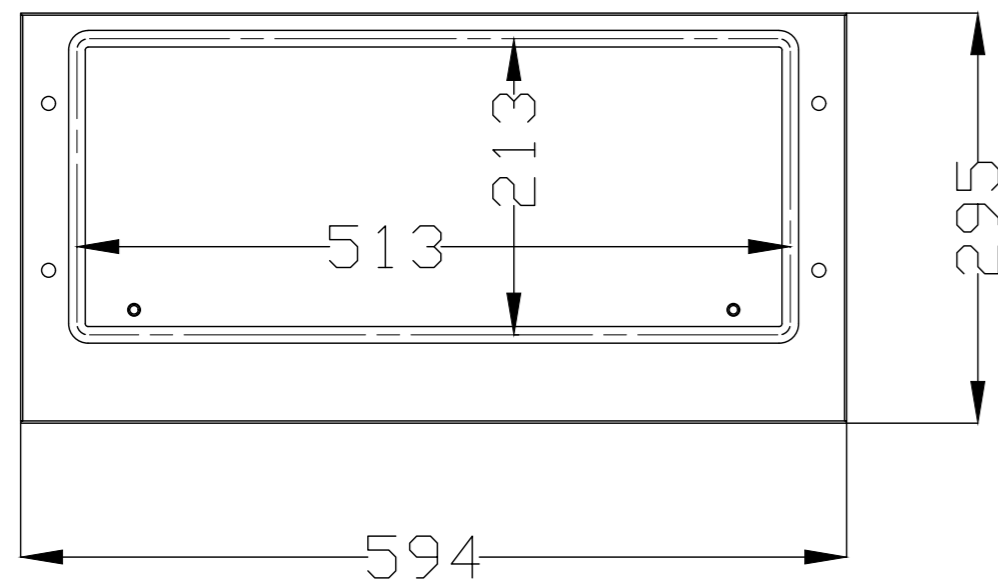
VISTA POSTERIOR PANEL FRONTAL FRONTAL PANEL REAR VIEW
