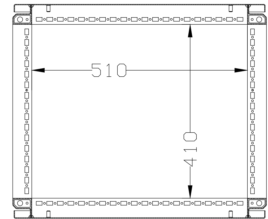
SEC. B-B
