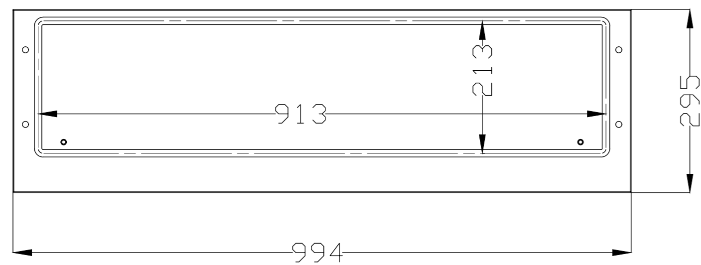
VISTA POSTERIOR PANEL FRONTAL FRONTAL PANEL REAR VIEW
