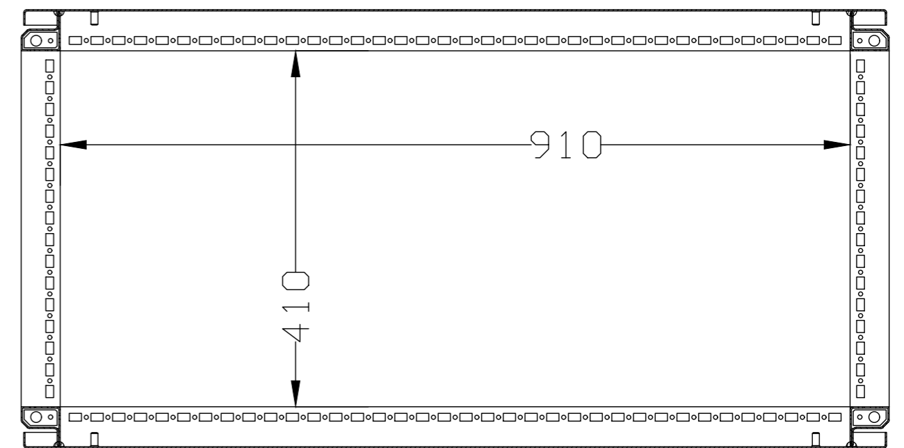
SEC. B-B
