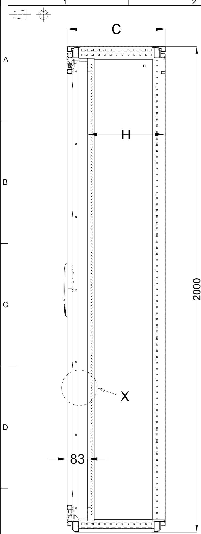
SEC. A-A'
