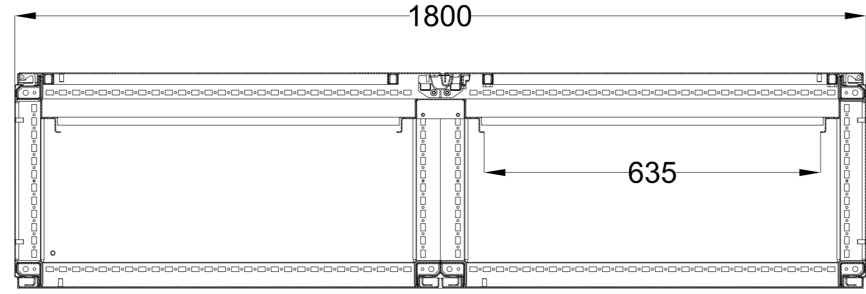
SEC. B-B'
