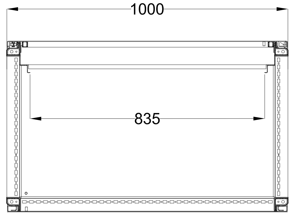
SEC. B-B'
