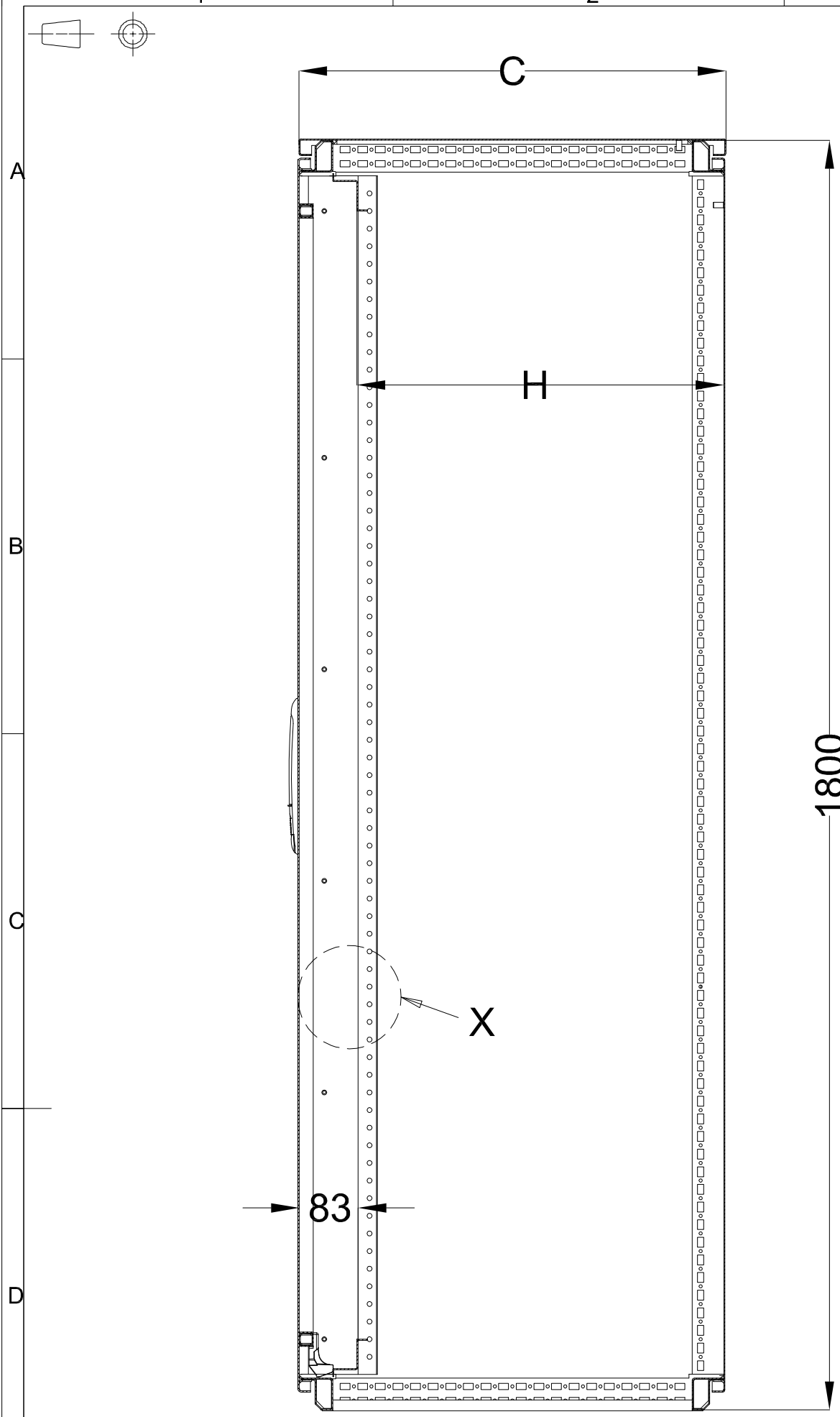
SEC. A-A'
