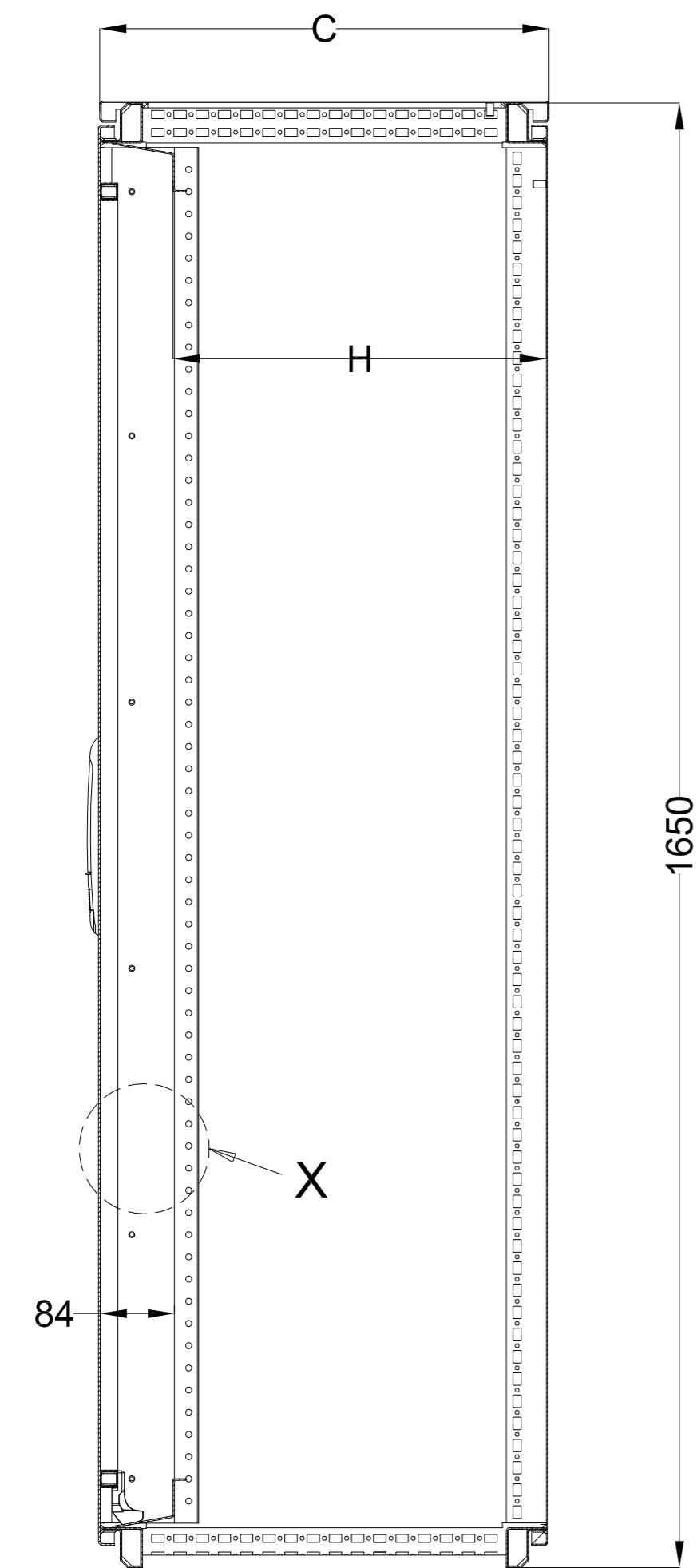
SEC. A-A'
