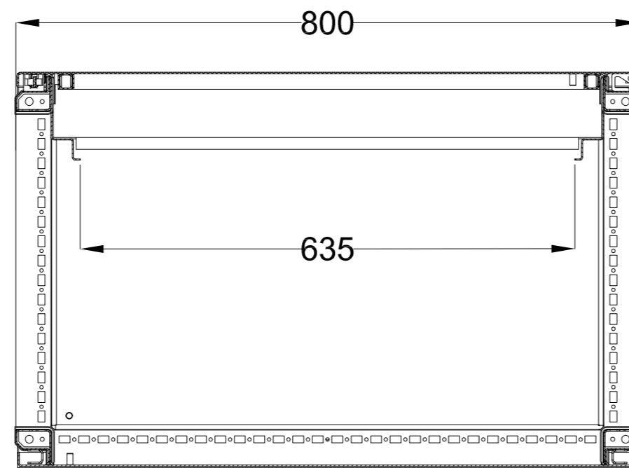
SEC. B-B'
