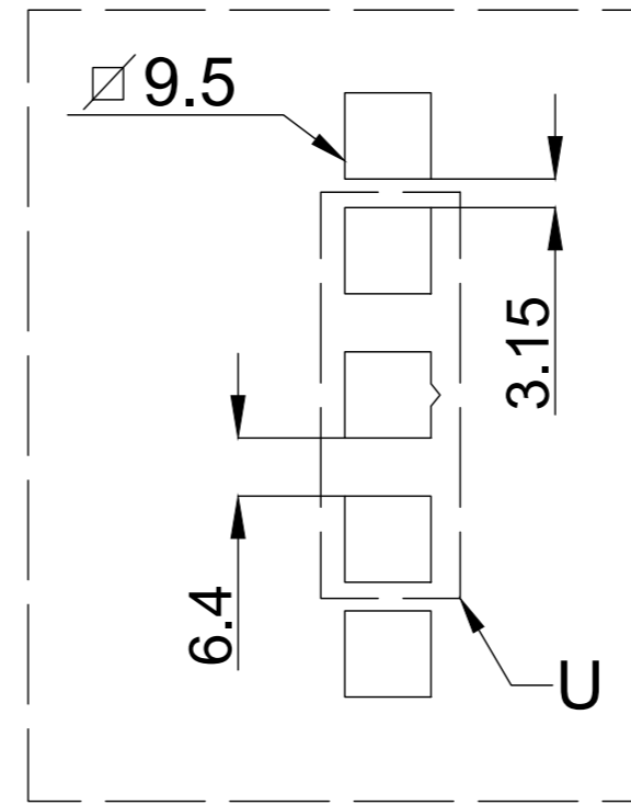
DETALLE X X DETAIL
