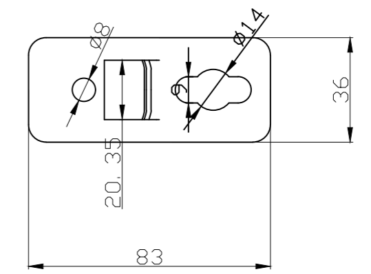
WALL MOUNTING SUPPORT (Ref.48463) SOPORTE A PARED (Ref.48463)
